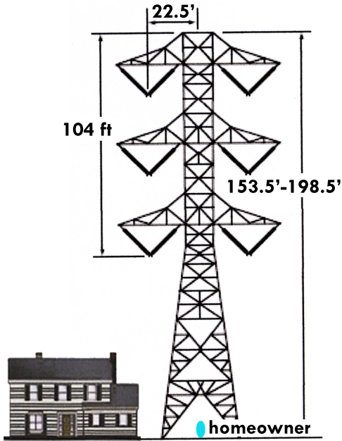
500 kV double circuit Lattice Steel Tower
